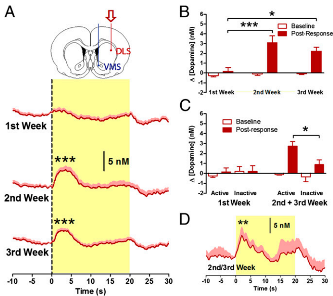
Fig. 3. Dopamine signaling in DLS over the course of weeks. (A) Phasic dopamine release in the DLS following responses into the active nose-poke port was observed during the second and third weeks of cocaine self-administration ( n = 15 ). (B) Dopamine signals in the second and third weeks were greater in amplitude than those in the first week. (C) Dopamine signals following responses into the active nose-poke port were larger than signals following inactive responses during the second and third weeks but not during the first week. (D) Noncontingent delivery of the CS induced dopamine release. * P < 0.05 , ** P < 0.01 , *** P < 0.001 .
