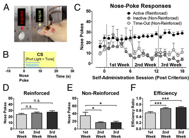
Fig. 1. Drug-taking behavior over the course of weeks. (A) Depiction of a rat connected to voltammetric recording equipment and infusion pump for i.v. delivery of cocaine during an approach to the active nose-poke port in the operant chamber. (B) A nose poke (dashed line) into the active port elicits an infusion of cocaine (0.5 mg/kg per infusion) and the presentation of a CS (yellow box) during a 20-s time-out. (C) Nose pokes into the active port, inactive port, and during the time-out period over 20 d of self-administration ( n = 18 ). (D) The number of reinforced nose pokes did not change significantly across weeks, whereas the number of nonreinforced responses decreased (E), and the ratio of reinforced over total number of nose pokes (efficiency) increased (F) in the second and third weeks compared with the first week. * P < 0.05 , *** P < 0.001 ; n.s., not significant.
