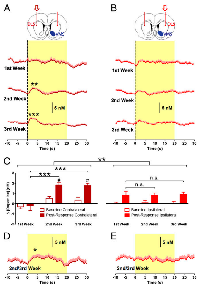
Fig. 5. VMS lesion prevents development of phasic dopamine signaling in the DLS. (A) Phasic dopamine release was observed in the DLS contralateral to the unilateral lesion of the VMS following responses into the active nose-poke port during the second and third weeks of cocaine self-administration ( n = 17 ). (B) Dopamine release in the ipsilateral DLS was not significantly increased in any week ( n = 11 ). (C) In the contralateral DLS, phasic signaling in the second and third weeks was larger in amplitude than signals detected in the first week (Left), whereas signals did not change in amplitude across weeks in the ipsilateral DLS (Right). Emergence of such signaling had significantly different patterns of dopamine release between hemispheres. A direct post hoc comparison between ipsilateral and contralateral hemispheres showed greater dopamine release in the contralateral hemisphere in the second and third weeks of training but not in the first week ( ^{\#}P < 0.05 ). (D and E) Noncontingent delivery of the CS consistently induced DLS dopamine release contralateral (D) but not ipsilateral (E) to the VMS lesion. *P < 0.05 , **P < 0.01 , ***P < 0.001 .
