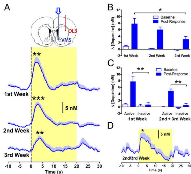
Fig. 2. Dopamine signaling in the VMS over the course of weeks. (A) Phasic dopamine release in the VMS following responses into the active nose-poke port was observed during all 3 wk of cocaine self-administration ( n = 10 ). (B) Dopamine signals decreased in amplitude over the course of 3 wk. (C) Dopamine signals following responses into the active nose-poke port were larger than signals following inactive responses. (D) Noncontingent delivery of the CS induced dopamine release. * P < 0.05 , ** P < 0.01 , *** P < 0.001 .
