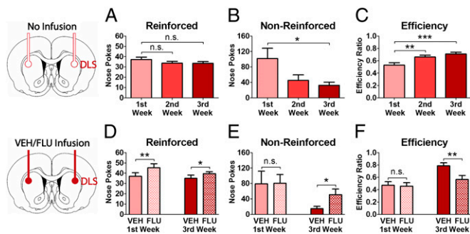
Fig. 4. Blockade of dopamine receptors in the DLS disrupts discriminated drug-taking behavior. (A–C) The rate of reinforced nose pokes remained stable across weeks (A), but the rate of nonreinforced nose pokes was decreased (B), and response efficiency increased (C) during the second and third weeks compared with the first week. (D) Infusion of flupenthixol (FLU) into the DLS produced an increase in reinforced nose pokes in both the first ( n = 16 ) and the third weeks ( n = 16 ). (E) The average number of nonreinforced responses was increased after flupenthixol only during the third but not during the first week. (F) Consequently, response efficiency was decreased after flupenthixol at the late but not at the early time point. * P < 0.05 , ** P < 0.01 , *** P < 0.001 ; VEH, vehicle.
